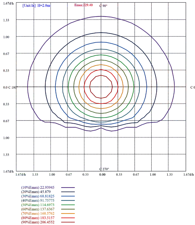
ISO illuminance diagram(Lux) of 5000K
