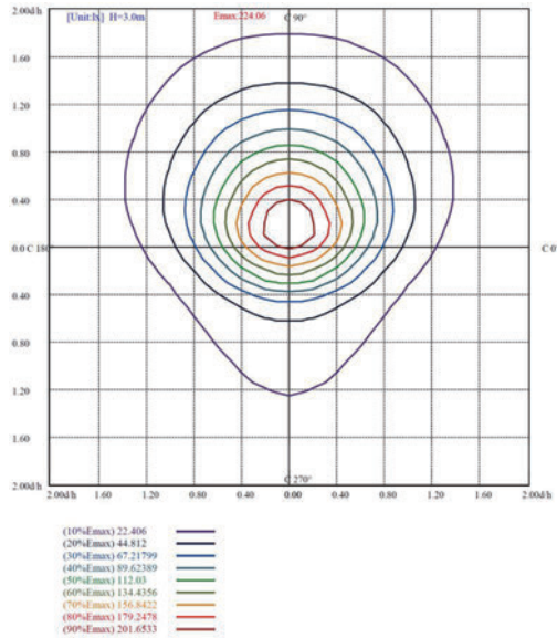
ISO illuminance diagram(Lux) of 3000K
