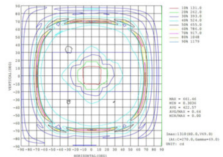
LASF isocandela Diagram
