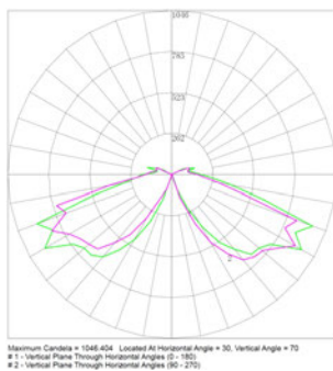
LARF/LARD Polar Curves of 3000K
