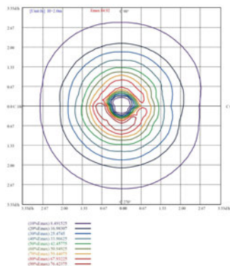
LARF/LARD Polar Curves of 3000K
