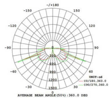
LASF Luminous Intensity Distribution
