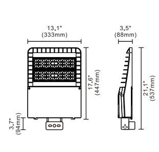
Trunnion Mount
