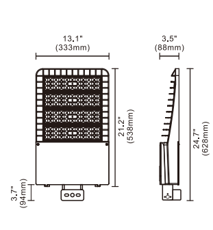
Trunnion Mount
