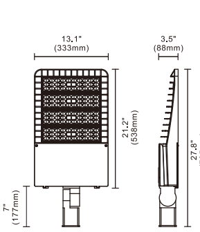
Knuckle Mount
