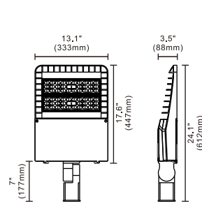
Knuckle Mount
