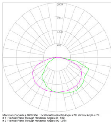
25 to 55W Polar Curves 3000K
