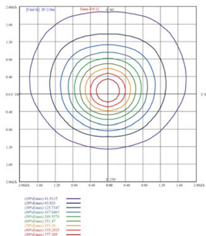
25 to 55W ISO illuminance diagram(Lux) 3000K
