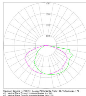
60 to 110W Polar Curves 3000K
