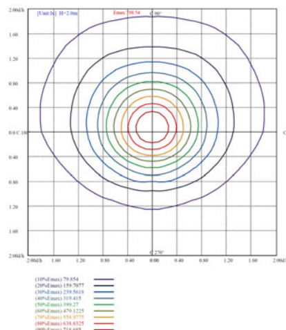
60 to 110W ISO illuminance diagram(Lux) 3000K
