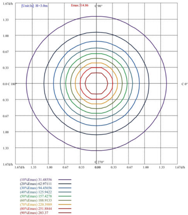
ISO illuminance diagram(Lux) of 3000K
