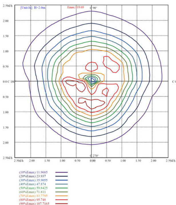
ISO illuminance diagram(Lux) of 3000K
