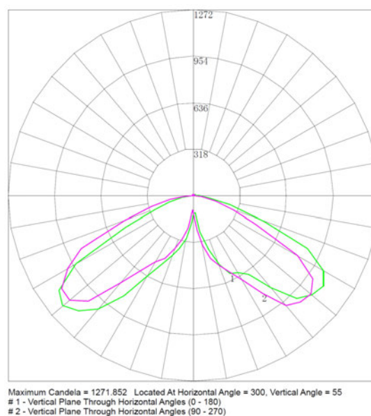
Polar Curves of 3000K
